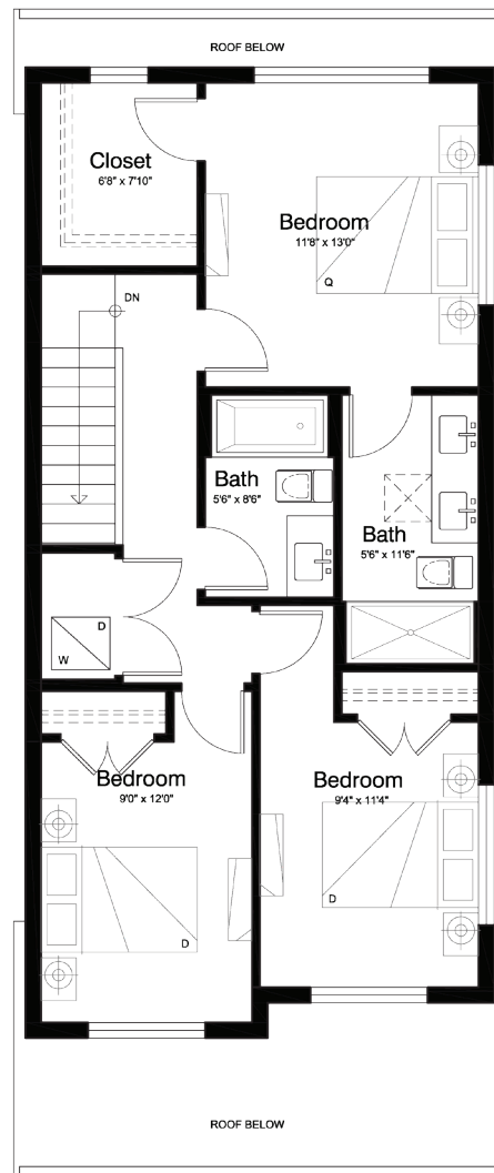
UPPER / 2ND FLOOR PLAN
