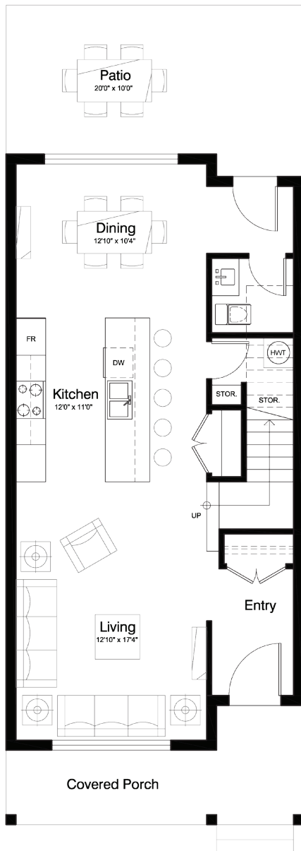
GROUND / 1ST FLOOR PLAN
